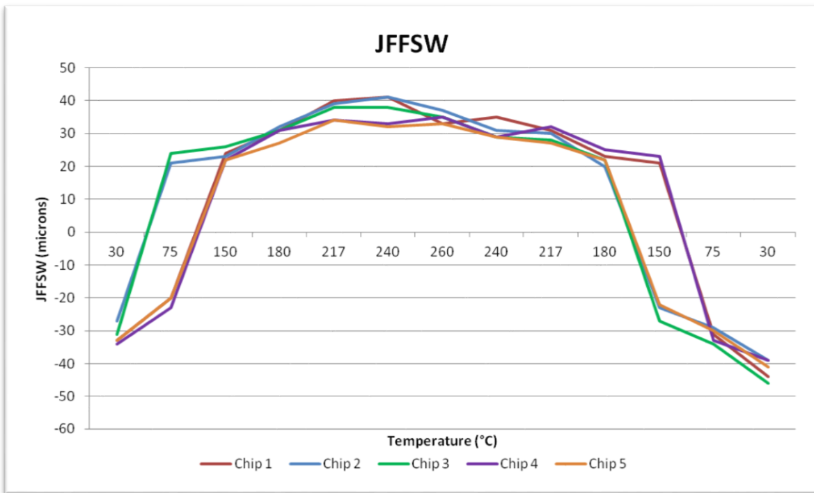
Figure 3. JFFSW, 5 Chip on Board Samples
