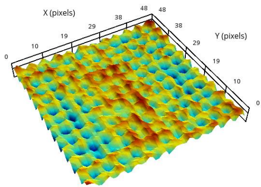
JFFS Warpage = 21 microns Figure 2a. CoB Sample 1, 150°C Cooling
