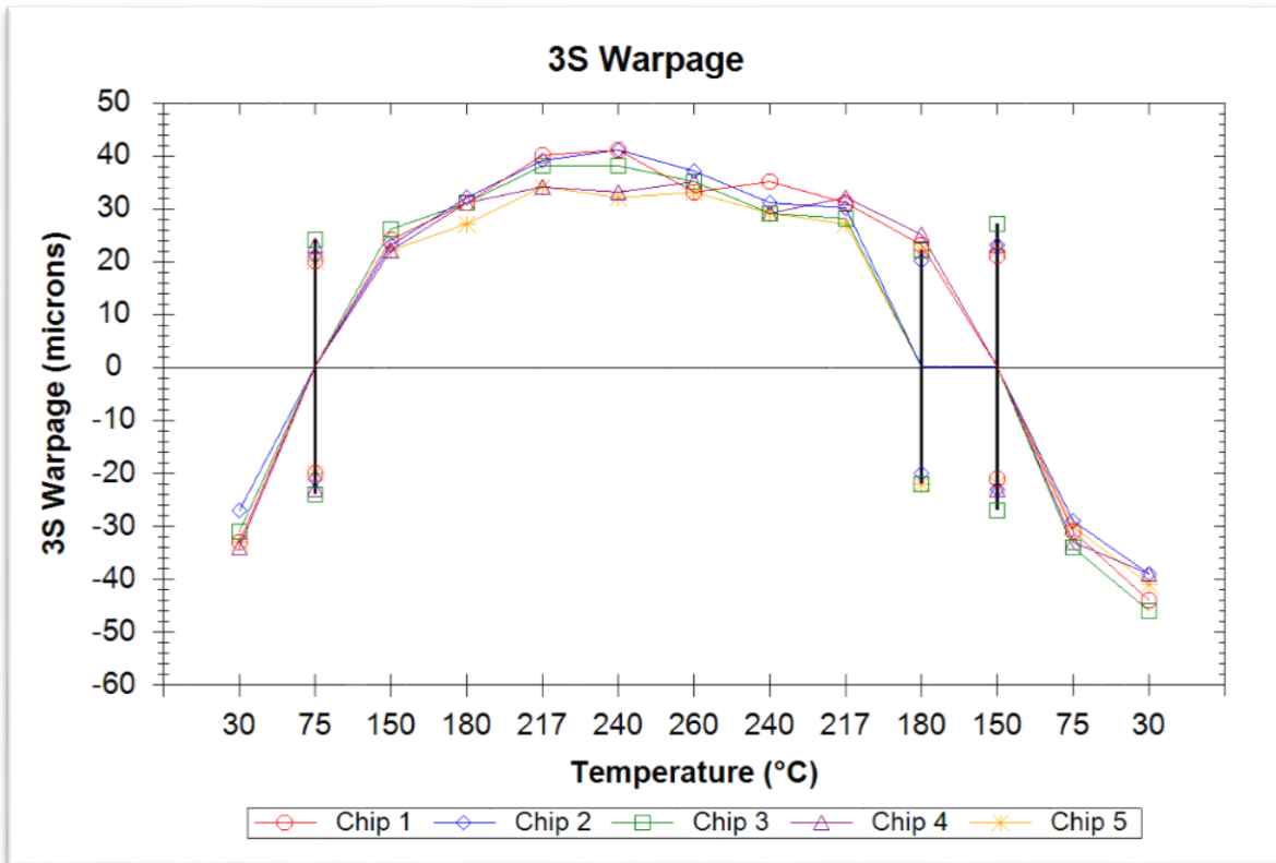
Figure 4. 3S Warpage, 5 Chip on Board Samples
