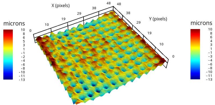
JFFS Warpage = -23 microns Figure 2b. CoB Sample 2, 150°C Cooling
